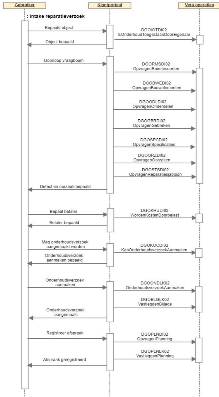
Sequence Diagram
